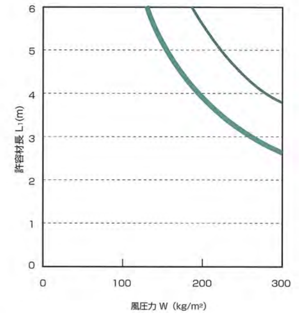
● L_2=4.0\text{m}
